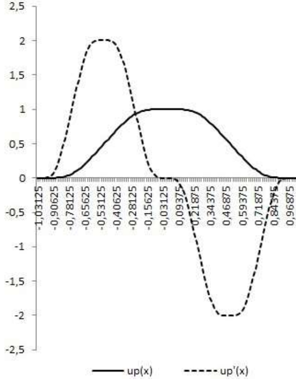
Fig. 1. The graph of up -function and its derivative
